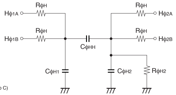
Horizontal transfer clock equivalent circuit
